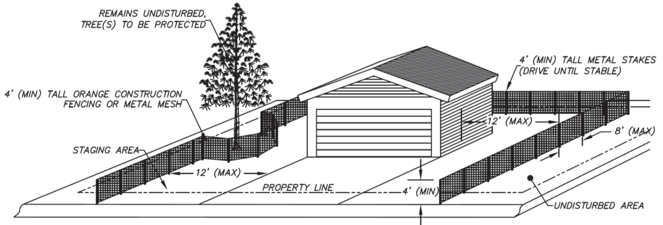
Figure 4.5-a: Construction Boundary Fencing
